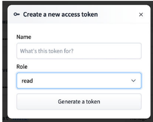
Figure 1-12. Huggingface token
