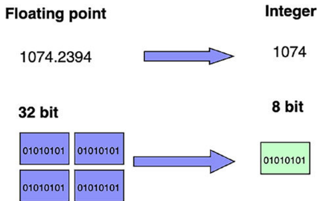
Figure 6-14. Quantization
