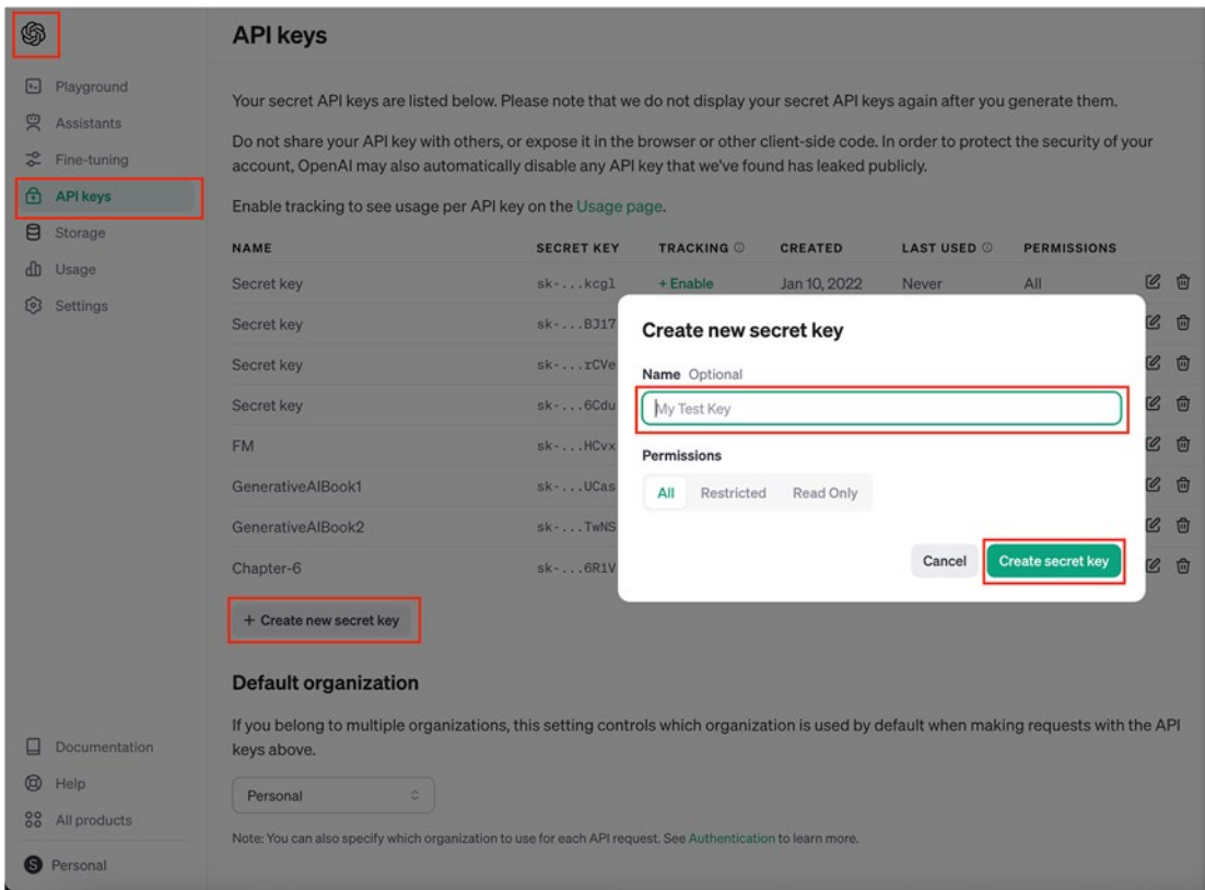
Figure 1-13. OpenAI token
