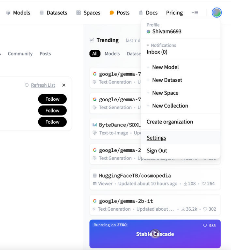
Figure 1-11. Huggingface account
