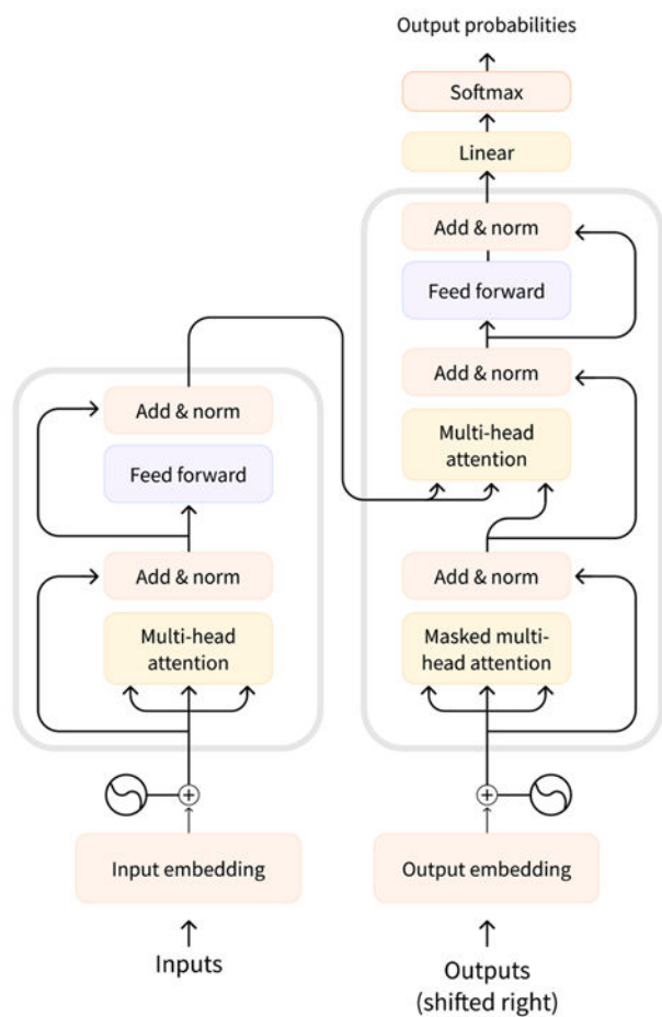
Figure 5-6. Original transformer architecture 14 (source: https://arxiv.org/pdf/1706.03762.pdf )
