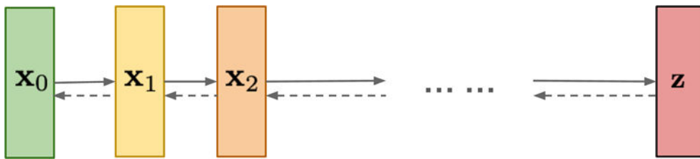
Figure 2-5. Diffusion models: gradually adding Gaussian noise and then reversing (source: https://lilianweng.github.io/posts/2021-07-11-diffusion-models/ )
