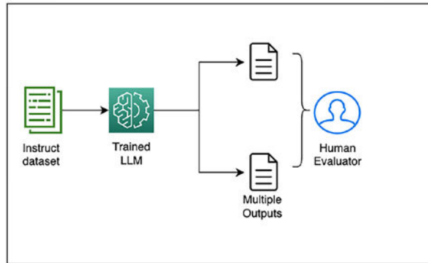
Figure 7-5. Reward model data collection
