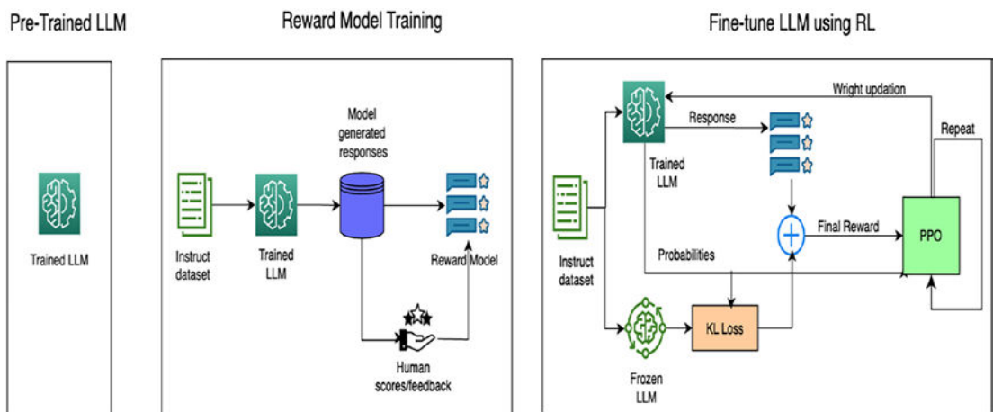
Figure 7-4. RLHF stages
