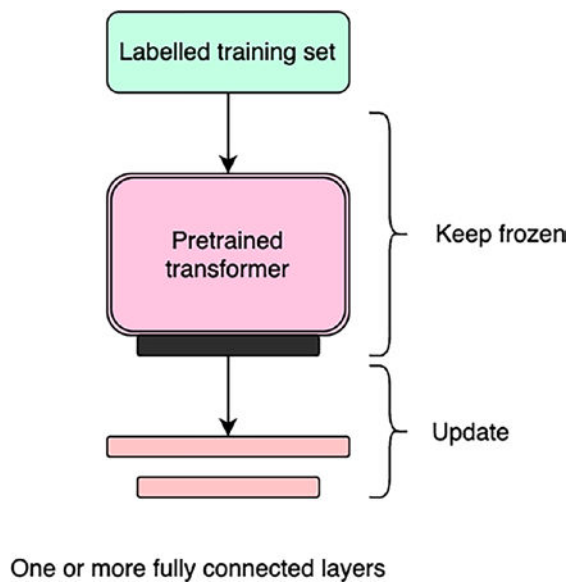
Figure 6-10. Fine-tuning LLM
