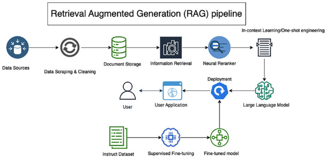
Figure 9-2. RAG architecture
