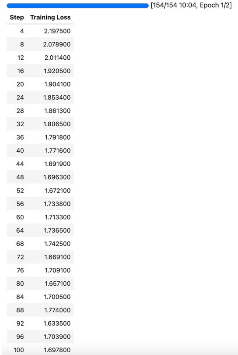
Figure 7-3. Llama2-7B fine-tuning
