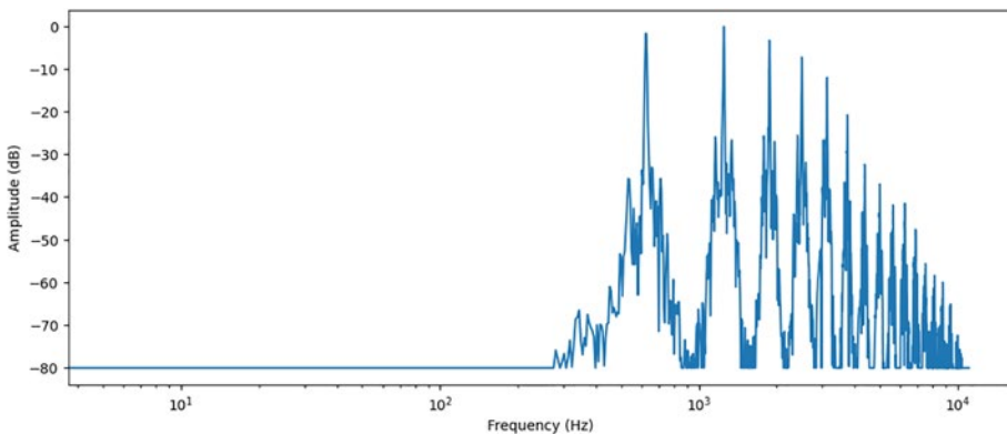
Figure 4-4. Plot of frequency spectrum
