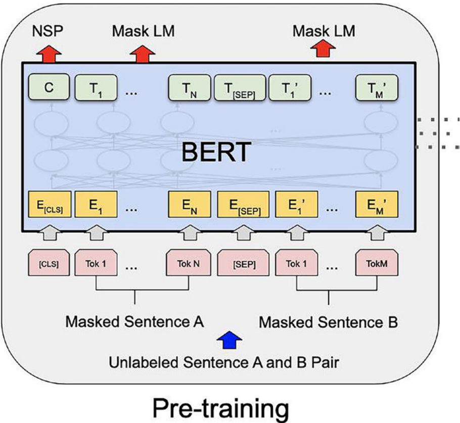
Figure 5-10. BERT pre-training 16 ( https://arxiv.org/abs/1810.04805 )
