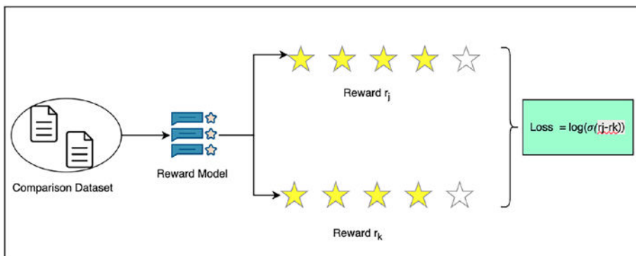
Figure 7-6. Reward model training
