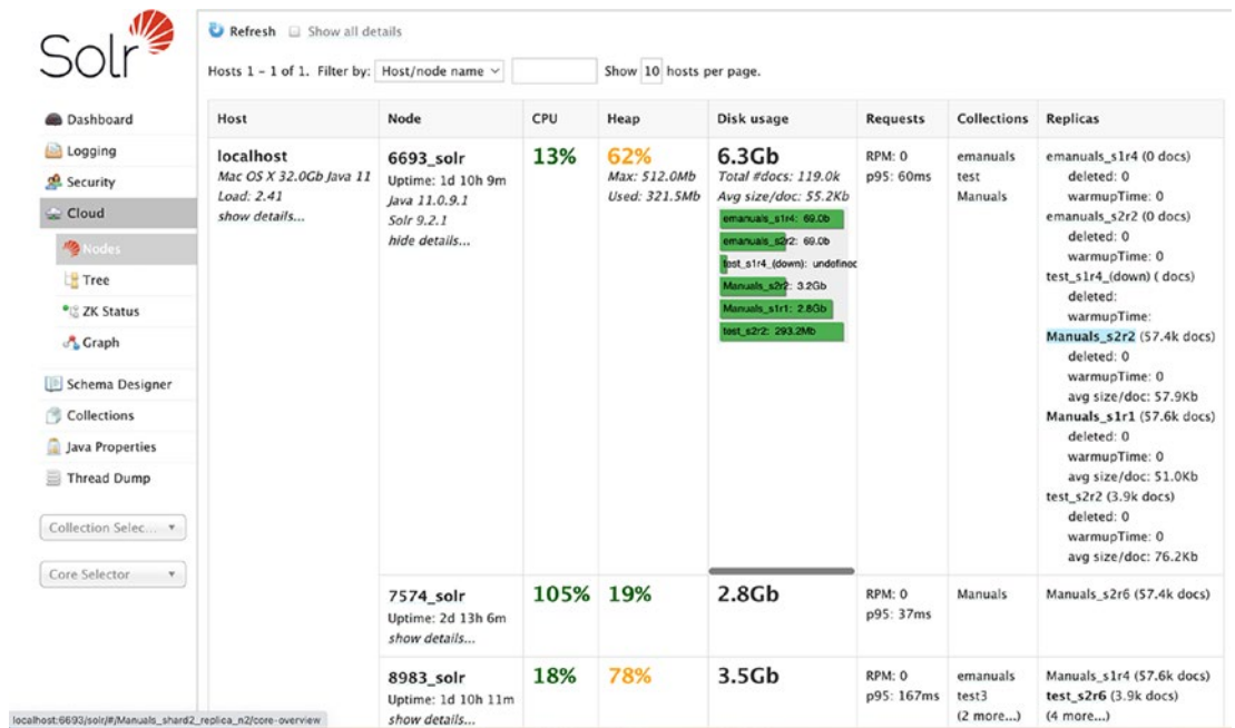
Figure 9-4. Solr Indexing UI
