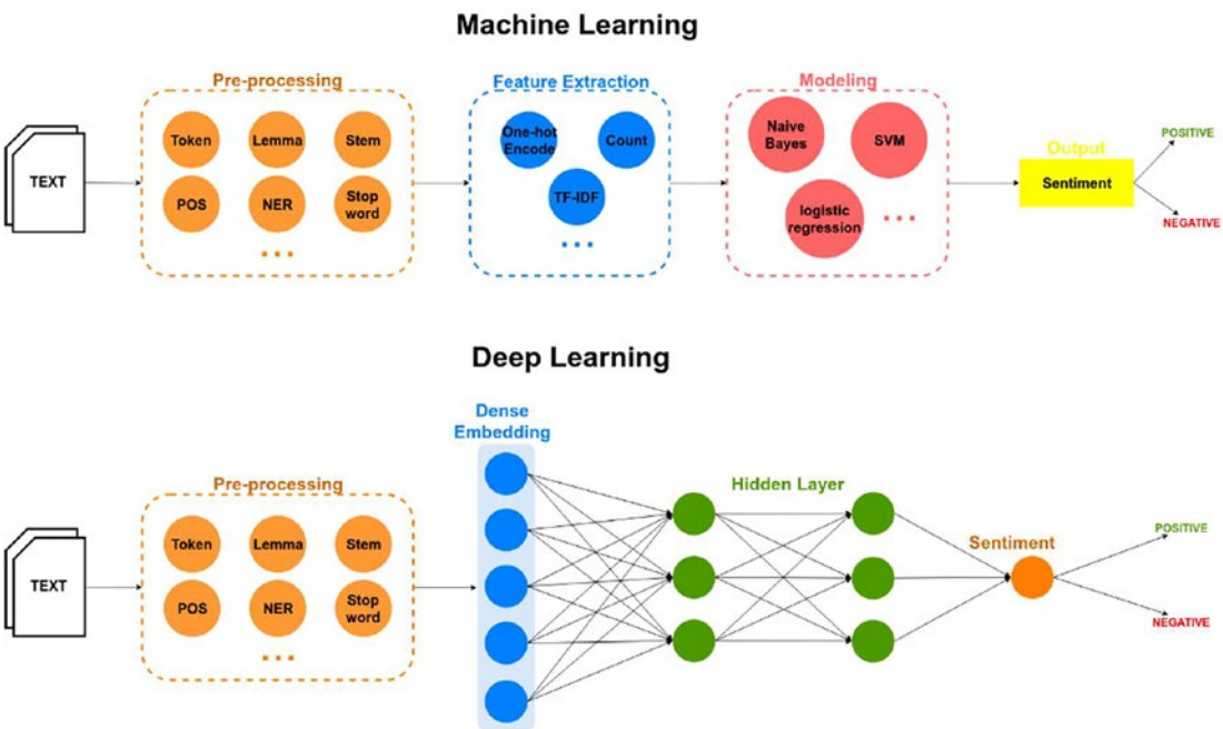
Figure 6-2. Sentiment analysis training procedure 23 (source: https://www.mdpi.com/2079-9292/9/3/483 )
