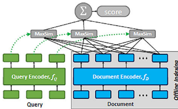
Figure 9-9. Colbert reranking (source: https://paperswithcode.com/paper/colbert-efficient-and-effective-passage )
