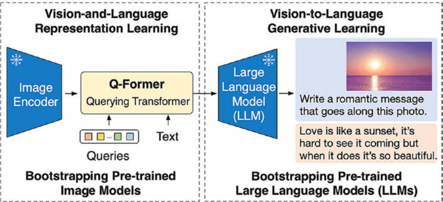
Figure 3-4. Flow of BLIP-2 (source: https://huggingface.co/blog/blip-2 )
