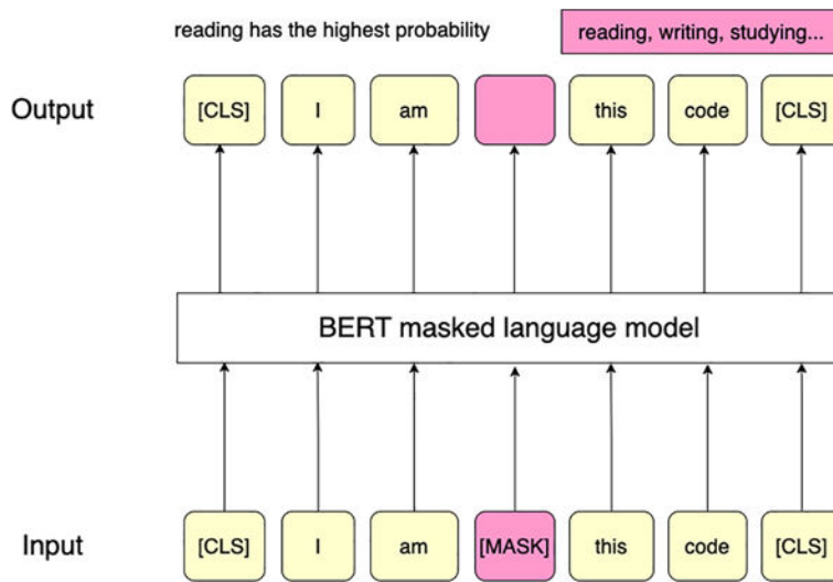
Figure 5-8. Masked language modeling
