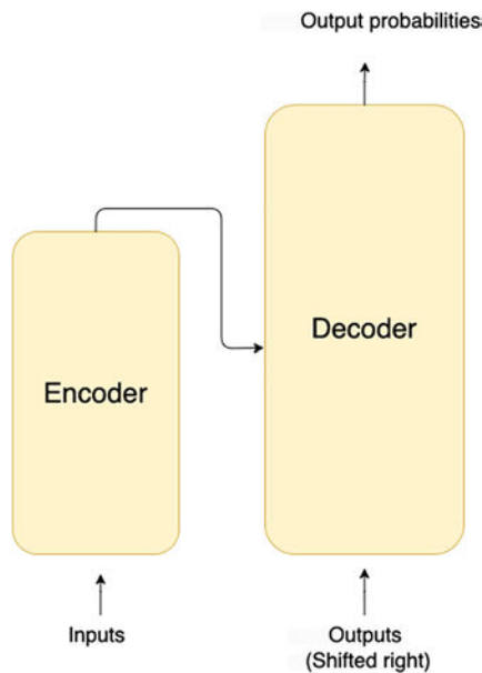
Figure 5-5. Basic language transformer architecture
