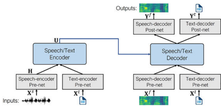
Figure 4-9. Architecture of SpeechT5 (source: arXiv:2110.07205 ) 10
