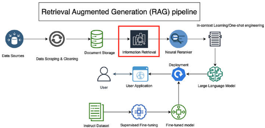
Figure 9-5. RAG information retrieval
