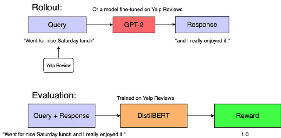
Figure 7-7. Reward tuning for LLMs
