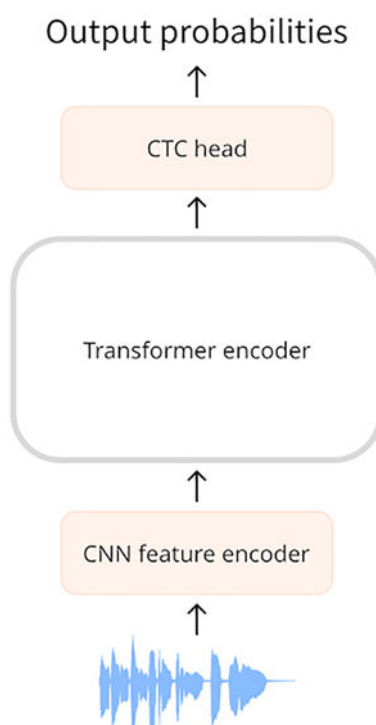
Figure 4-7. Flow for CTC architectures ( https://huggingface.co/learn/audio-course/chapter3/ctc )
