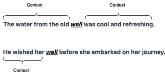
Figure 5-7. BERT’s bidirectional context approach
