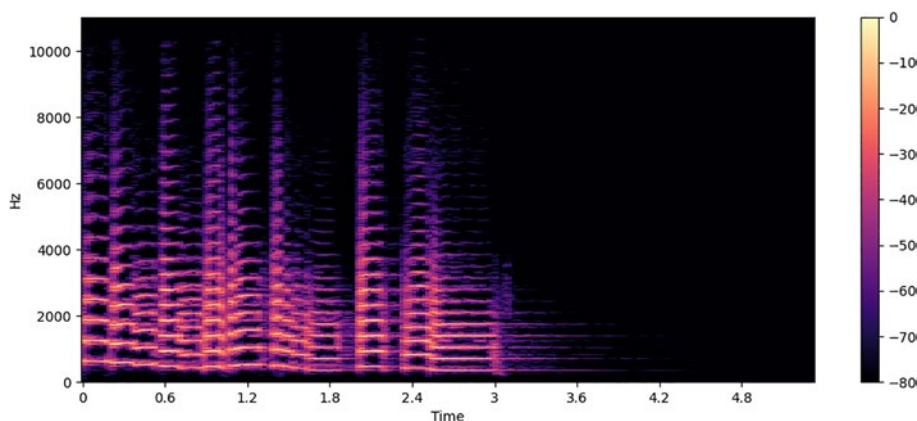
Figure 4-5. Plot of spectrogram
