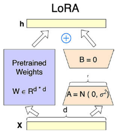
Figure 6-12. LoRA fine-tuning of LLM 26
