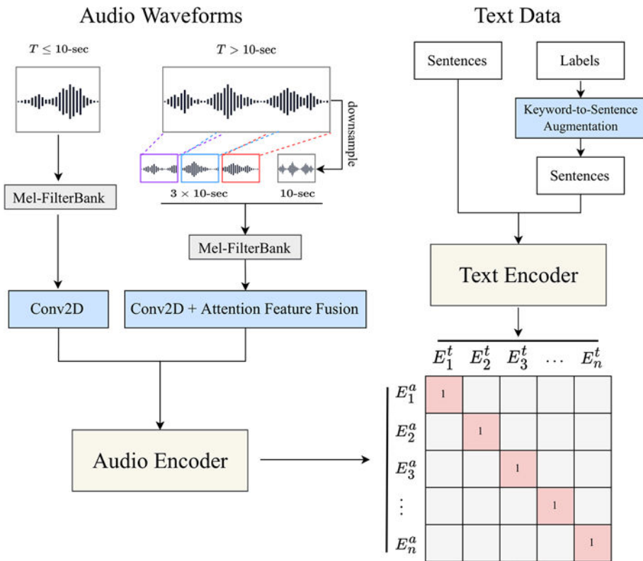
Figure 4-6. CLAP architecture 7 (source: https://github.com/LAION-AI/CLAP?tab=readme-ov-file )
