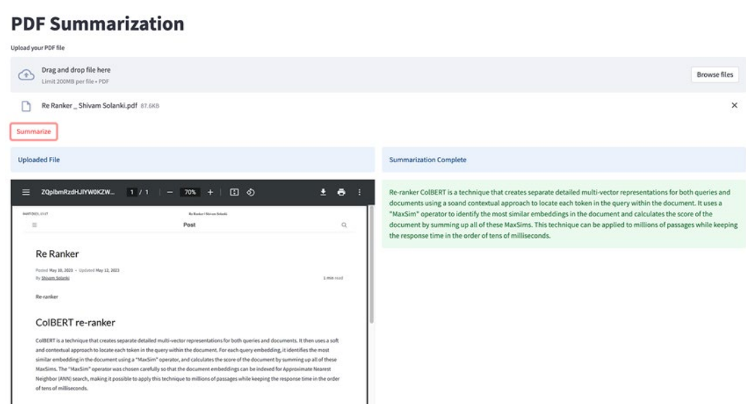
Figure 8-4. PDF summarization
