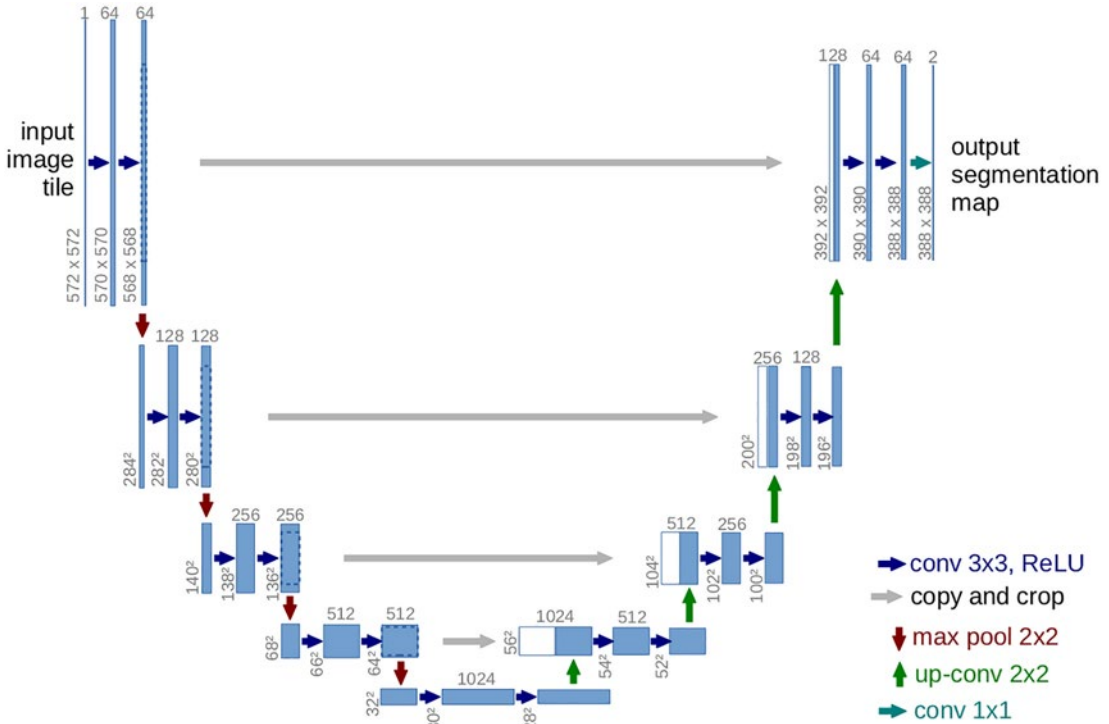
Figure 2-7. U-net architecture
