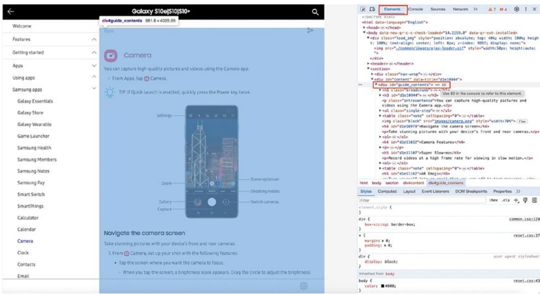
Figure 8-1. Website scraping
