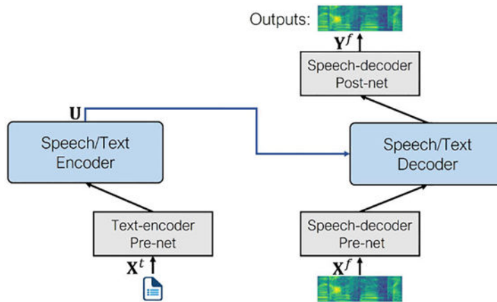
Figure 4-10. Architecture of SpeechT5 during fine-tuning (source: arXiv:2110.07205)
