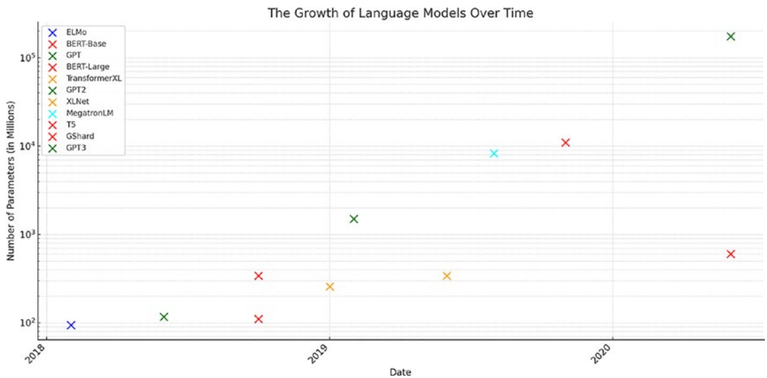
Figure 5-1. Growth of LLMs over time
