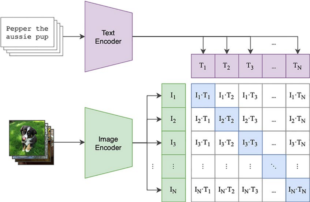
Figure 2-3. CLIP pre-training architecture (source: https://openai.com/research/clip )
