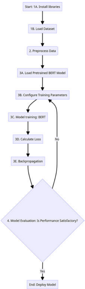
Figure 5-12. BERT fine-tuning flowchart
