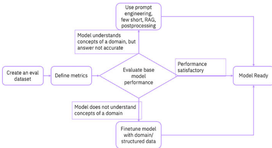
Figure 6-9. Fine-tuning decision flowchart
