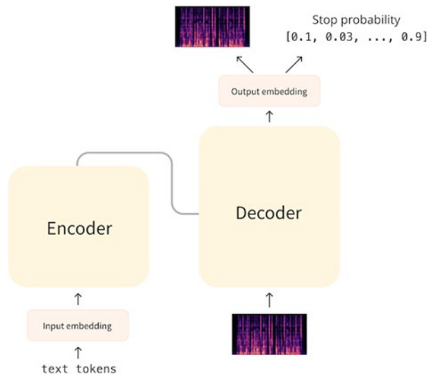
Figure 4-8. Flow of Seq2Seq architectures ( https://huggingface.co/learn/audio-course/chapter3/seq2seq )
