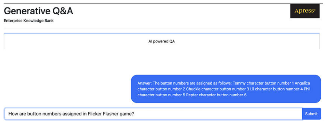
Figure 9-12. RAG UI
